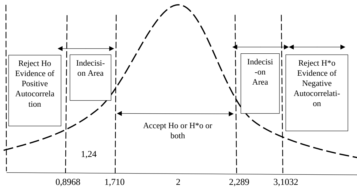
Figure 6. Autocorrelation Graph
